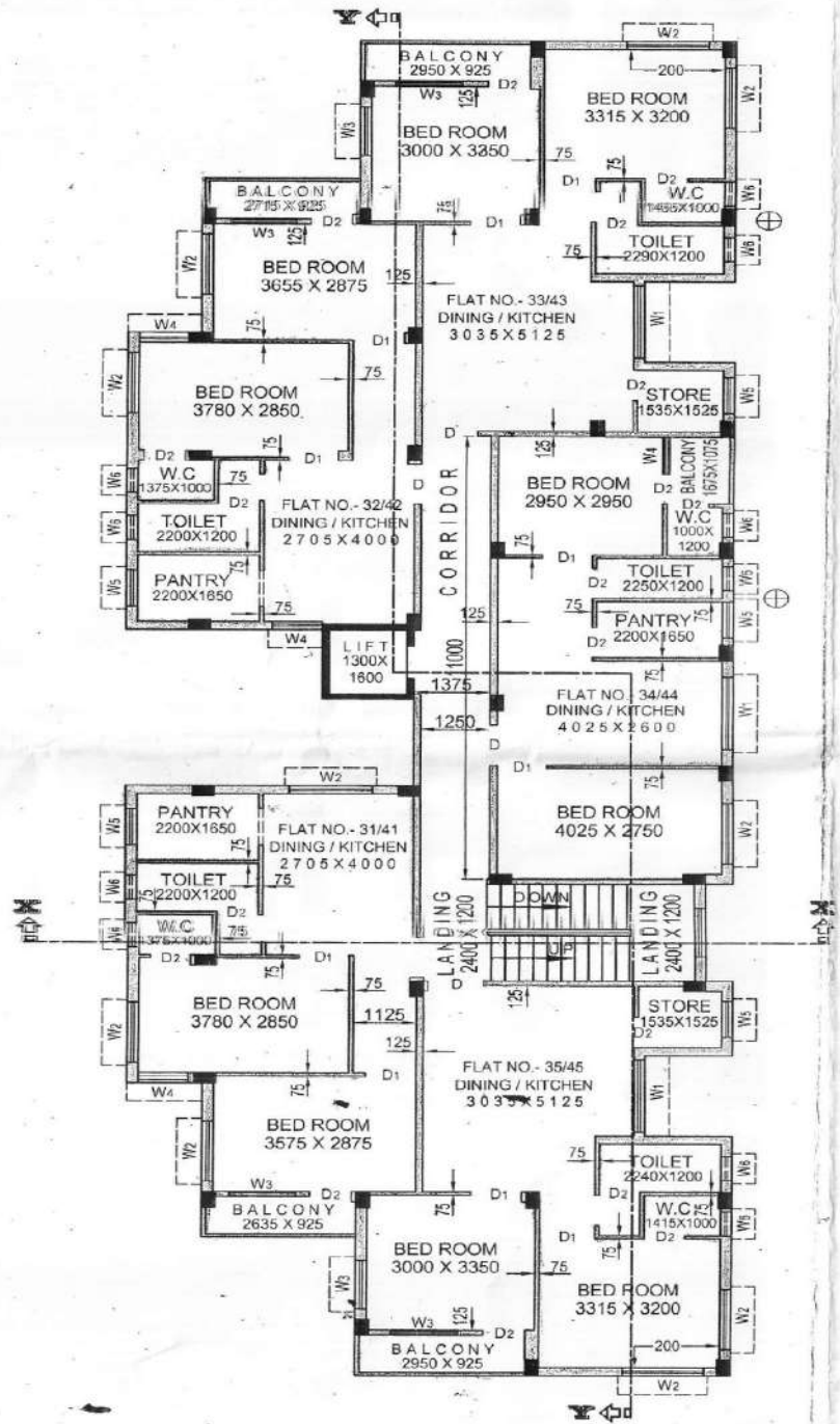
SECOND & THIRD FLOOR PLAN
